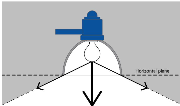
Figure 4-4: Example of Fully Shielded Light Fixture
