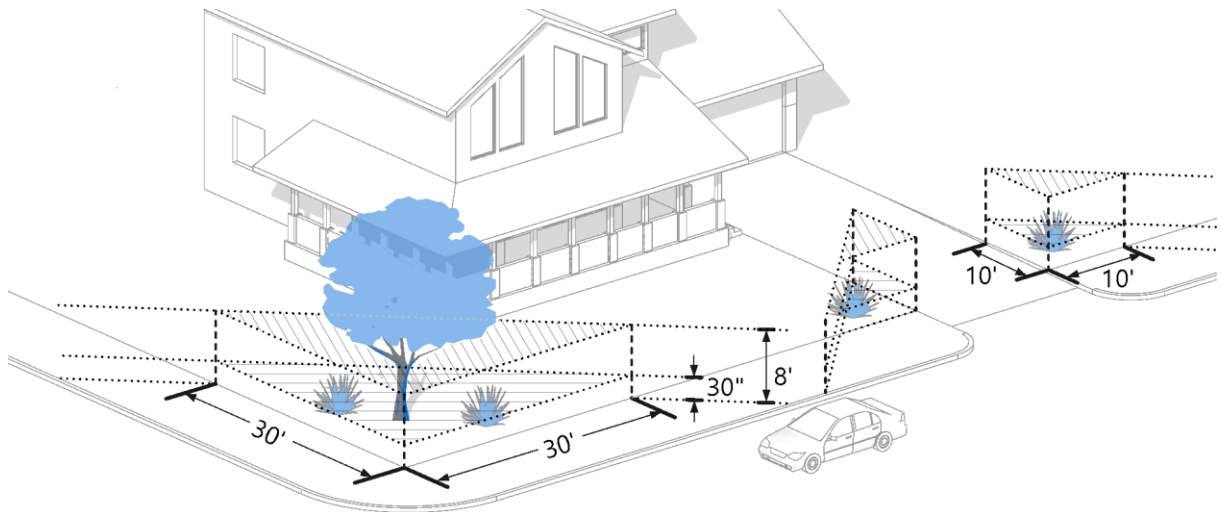
Figure 4-2: Visibility Triangle
